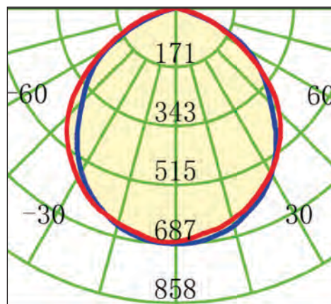
PHOTOMETRIC DIAGRAM
