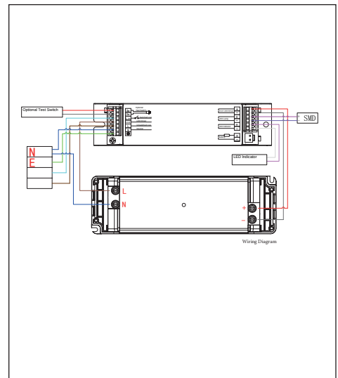
WIRING DIAGRAM
