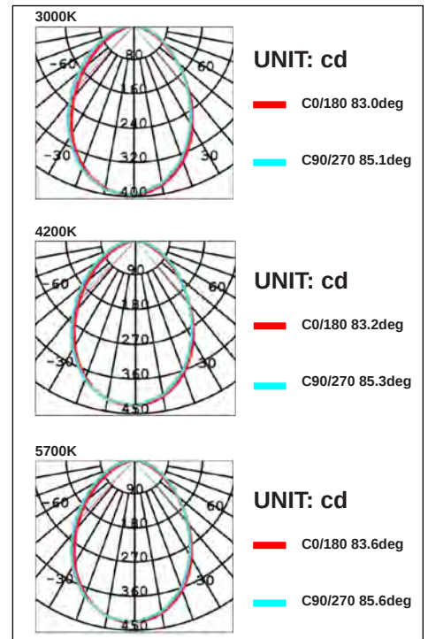
PHOTOMETRIC DIAGRAM
