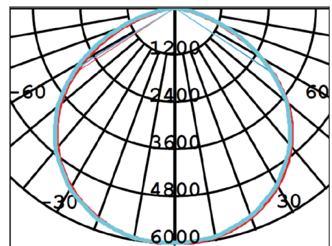
PHOTOMETRIC DIAGRAM
