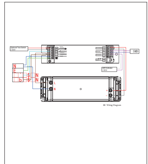
WIRING DIAGRAM
