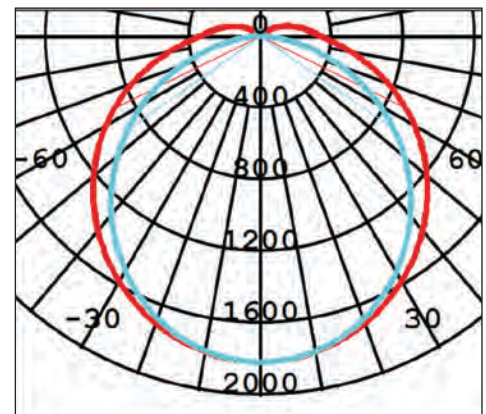
PHOTOMETRIC DIAGRAM
